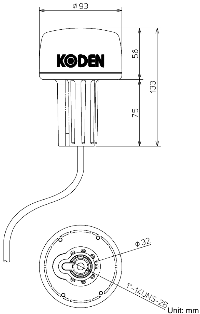
Figure 1.1 GPS-20A MkII external dimensions
