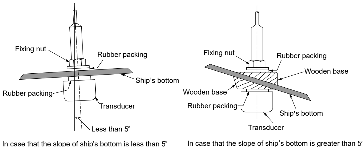
Figure 5.7 Through-hull Installation
