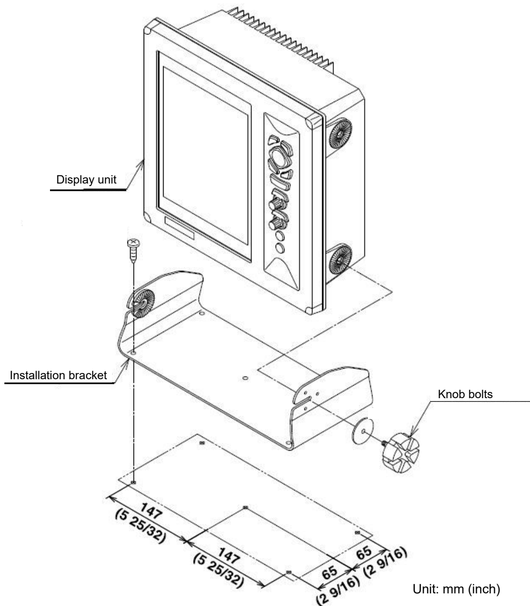
Fig. 5.2 Desk-top installation
