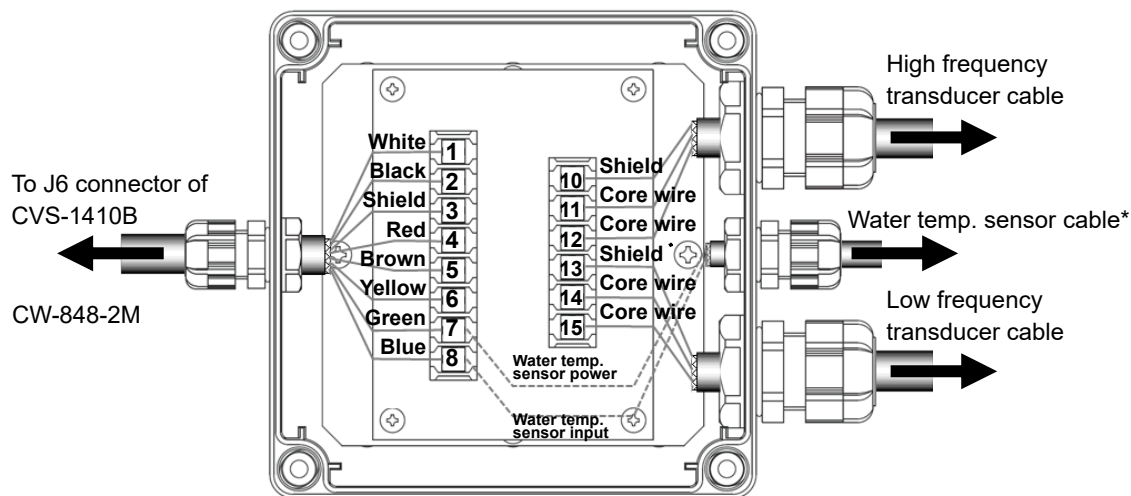
Connection of Transducer switching unit (JB-38)
