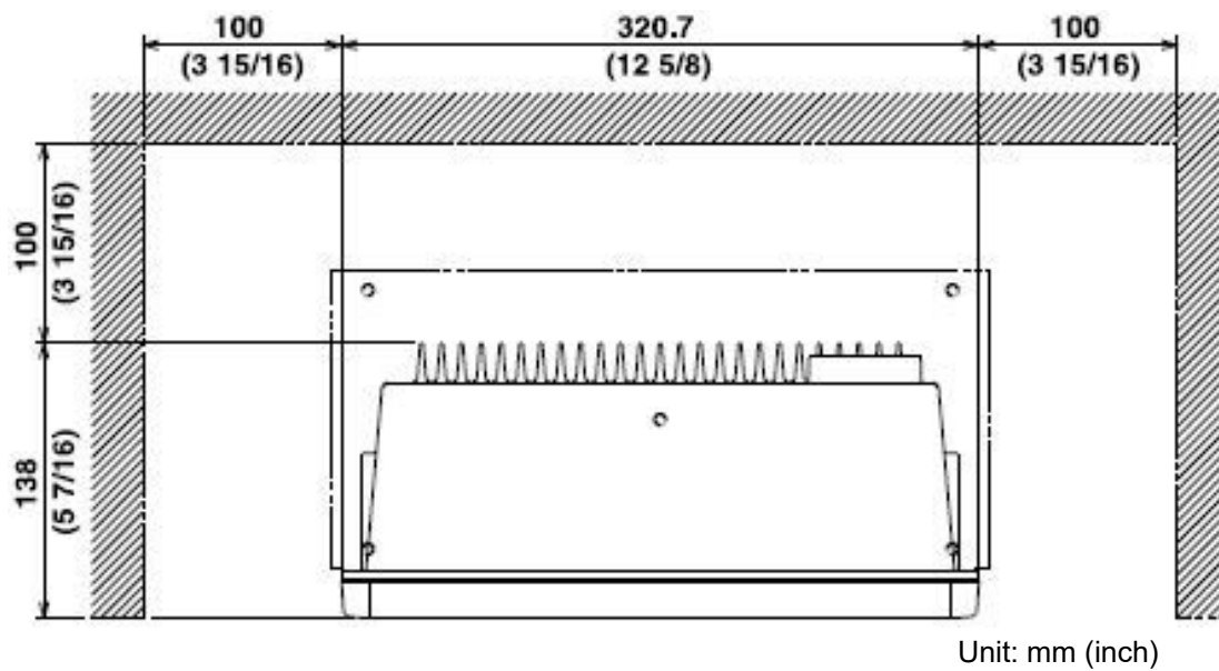
Fig. 5.3 Maintenance space
