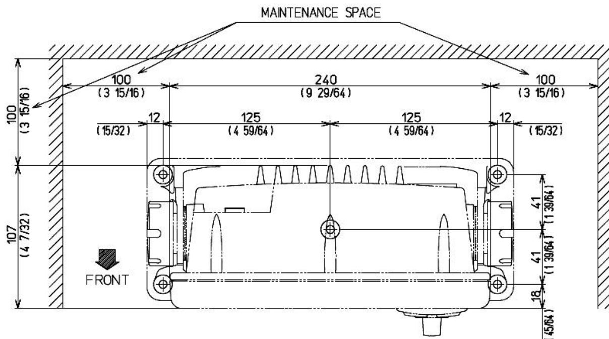
Fig. 5.3 Maintenance space
