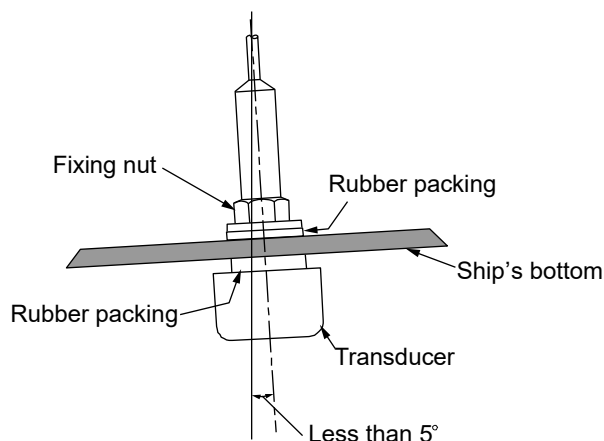
Figure 5.8 Through-hull Installation
