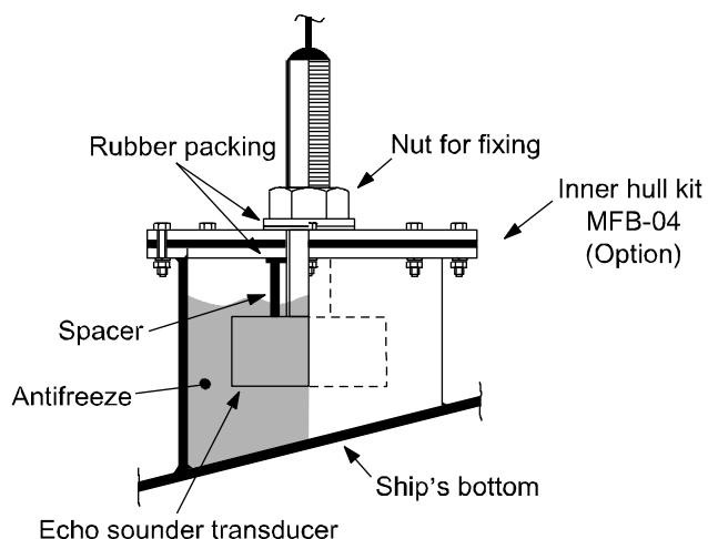
Figure 5.7 Inner-Hull installation
